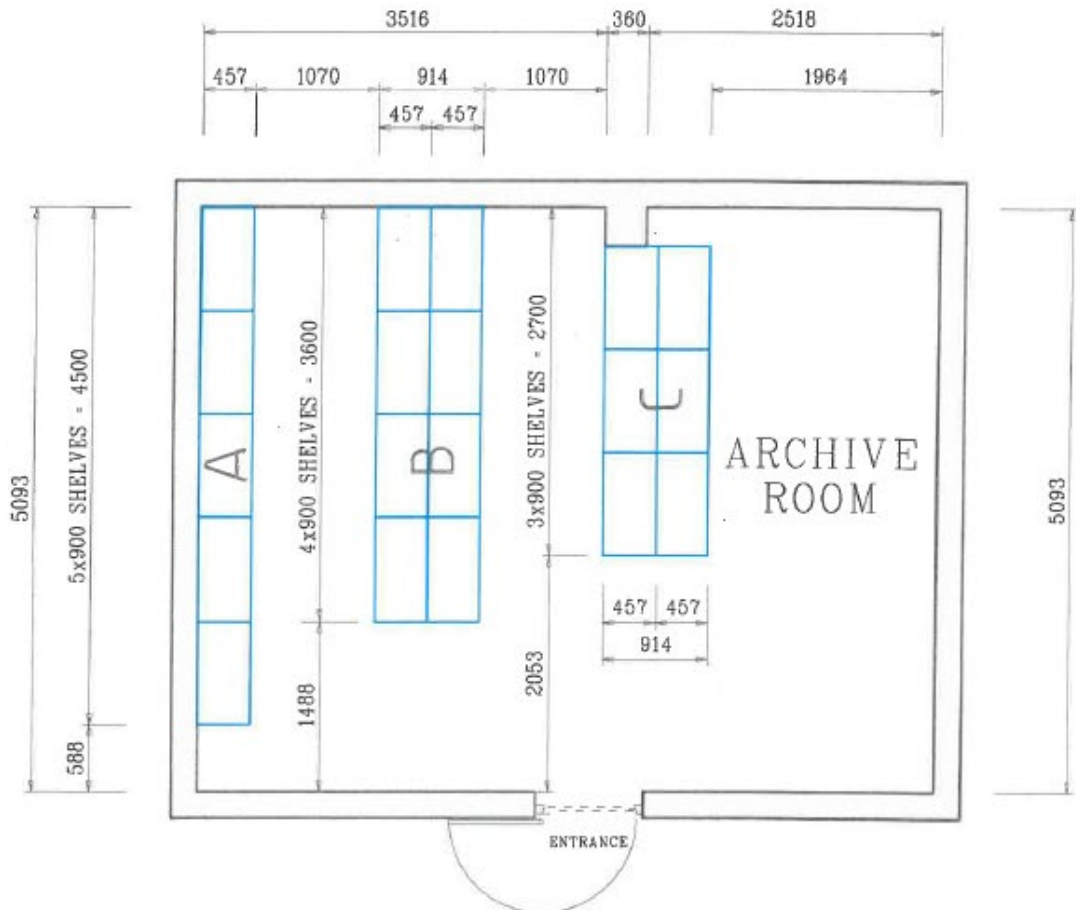
FLOOR PLAN 1:50
